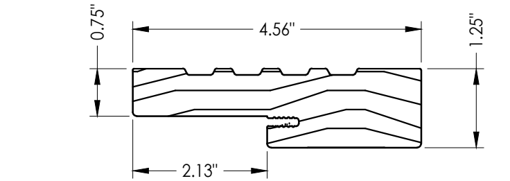
1 WOOD JAMB (4-9/16")
