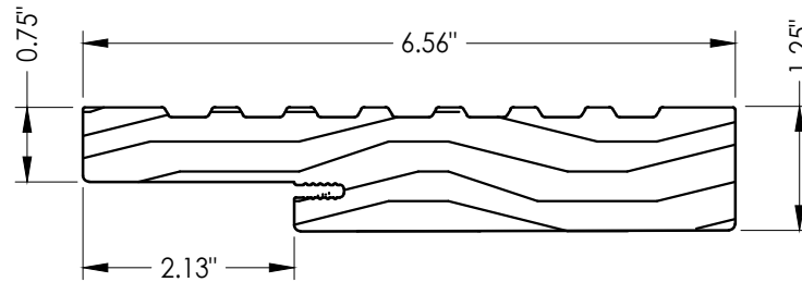
2 WOOD JAMB (6-9/16")
